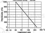
PRESSURE TEMPERATURE RATINGS 8NB ~ 50NB
