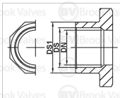
SOCKET WELD END
